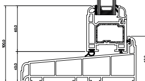
Sideways View - Standard Bottom Rail
